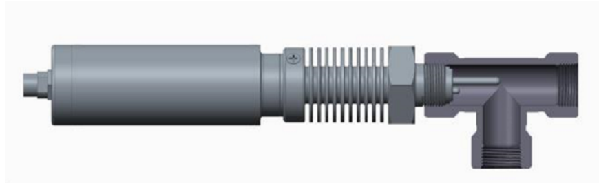
Figure 2. CR-301 Installation in the sample flow line
